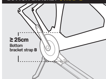
BOTTOM BRACKET STRAP B
